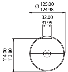
SHAFT END DETAIL
